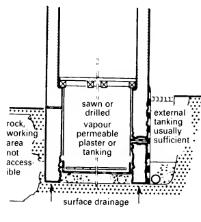
⑧ Retrofitted damp-proofing and drainage in cellar area
